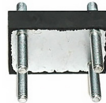
Z070 003 195 Shock Mount Sweep
